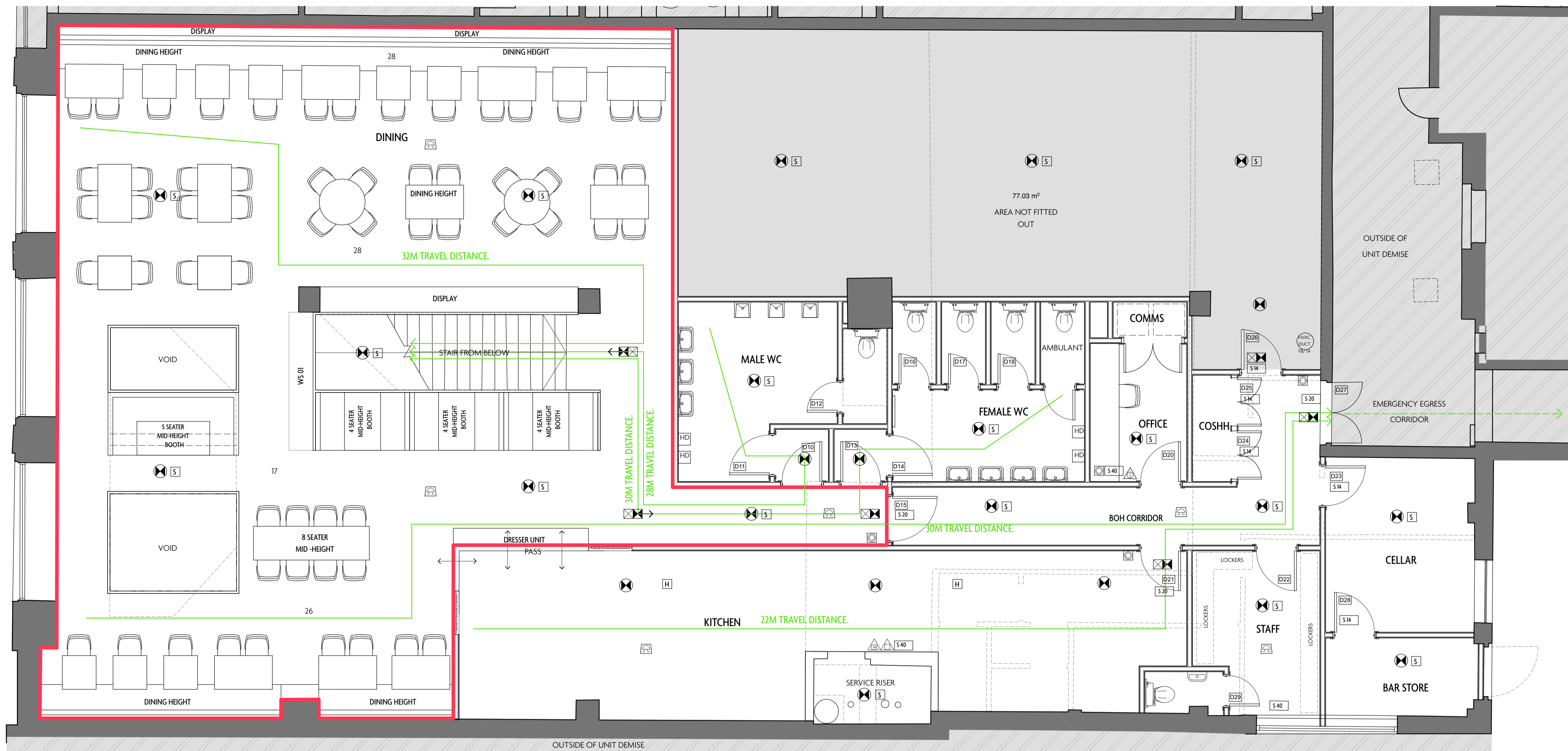
FIRST FLOOR GA SCALE 1:50 @ A1
